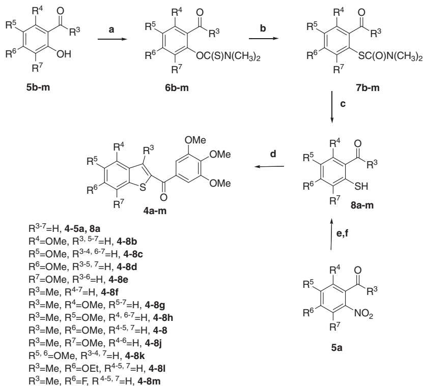
Scheme 1. Reagents and conditions. (a) ClC(S)N(CH 3 ) 2 , Dabco, DMF, 50 °C, 5 h; (b) no solvent, heating of fused substrates, microwaves; (c) NaOH, EtOH/H 2 O, 65 °C; (d) (3,4,5-trimethoxyphenyl)-2-bromo-ethanone, K 2 CO 3 , (CH 3 ) 2 CO, rx; (e) C 6 H 5 CH 2 SH, KOH, DMF; (f) AlCl 3 , C 6 H 6 .
