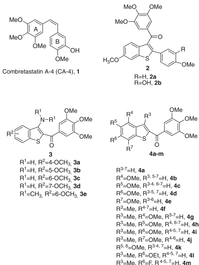
Chart 1. Inhibitors of tubulin polymerization.
